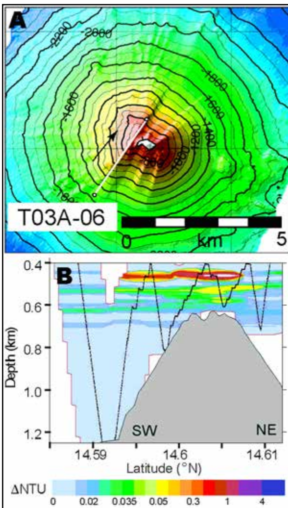
Plotted results of towed hydrocast over an underwater volcano
