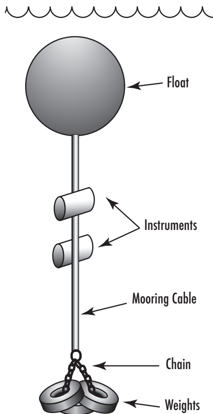
Figure 1: Mooring System
