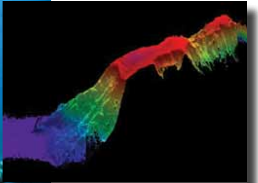
Partial bathymetry data for Kelvin Seamount Image by N. Forfinski
