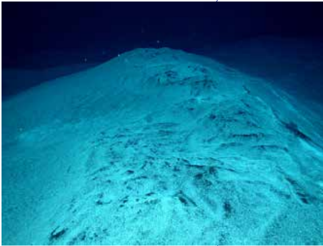
Microbial mats coated in white sulfate material were observed and sampled at several vent sites at West Mata in 2009. These mats were dominated by Epsilonproteobacteria which is a class of bacteria often associated with sulfur oxidation in marine environments. Image courtesy of NOAA /NSF/WHOI.
